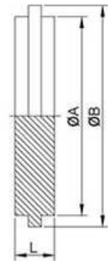
IDF-16AMP Blank
