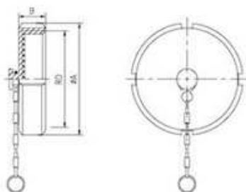
DIN blind nut with chain
