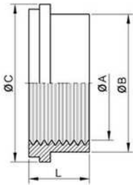
IDF-14R Expanding Liner
