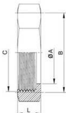
Hexagon Nut
