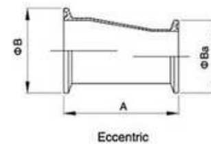
Eccentric
