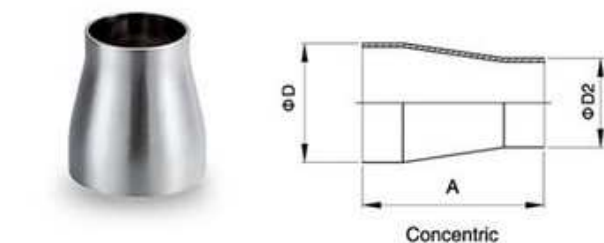
Welded Reducer
