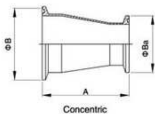
Concentric
