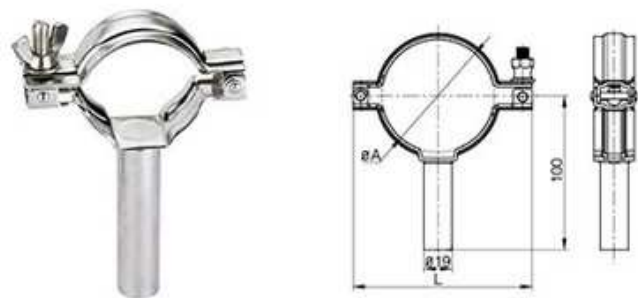
TH1H Pipe Holder(Welded)
